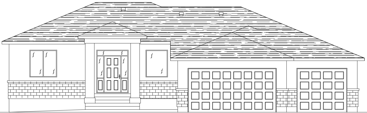
—FRONT ELEVATION—
